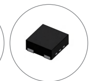
DFN1.6*1.6-6L(SM) 1.6*1.6*0.4
